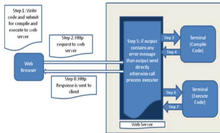
Figure 1: Architecture of Web Based IDE
